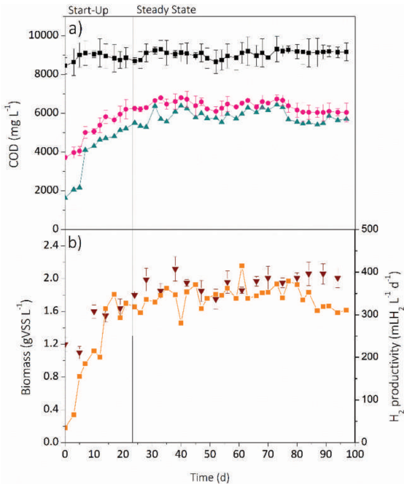
Figure III.3 Acidogenic fermentation reactor operation profile for 98 d. a) Shows TCOD (■), SCOD (●) and COD equivalent of all SCCA (▲). B) shows H 2 productivity (■) and biomass (▼) within in the reactor (b).
