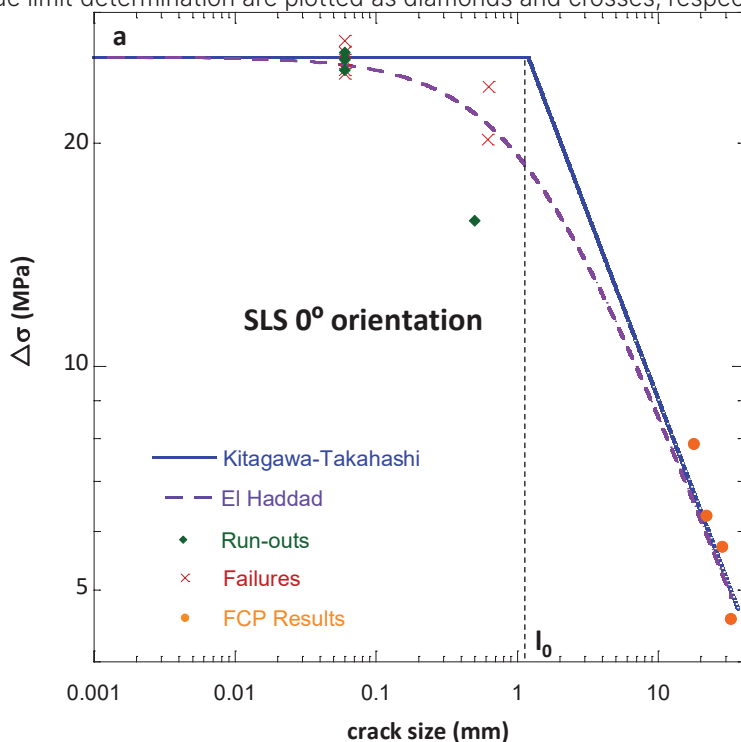
Figure 6-4. Kitagawa-Takahashi diagram (blue line) including El Haddad empirical model (purple line) of a) SLS PA-12 at 0° orientation, b) SLS PA-12 at 90° orientation and c) IM PA-12.ex Experimental data from \Delta\sqrt{G} -decreasing tests are plotted with orange filled circles, and the run-outs and failures of the tests employed for the fatigue limit determination are plotted as diamonds and crosses, respectively.
