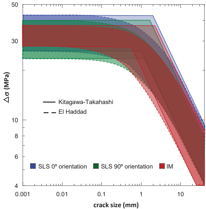
Figure 6-10. Schematic Kitagawa-Takahashi of SLS PA-12 at 0° orientation in blue, SLS PA-12 at 90° orientation in green and IM PA-12 in red.
