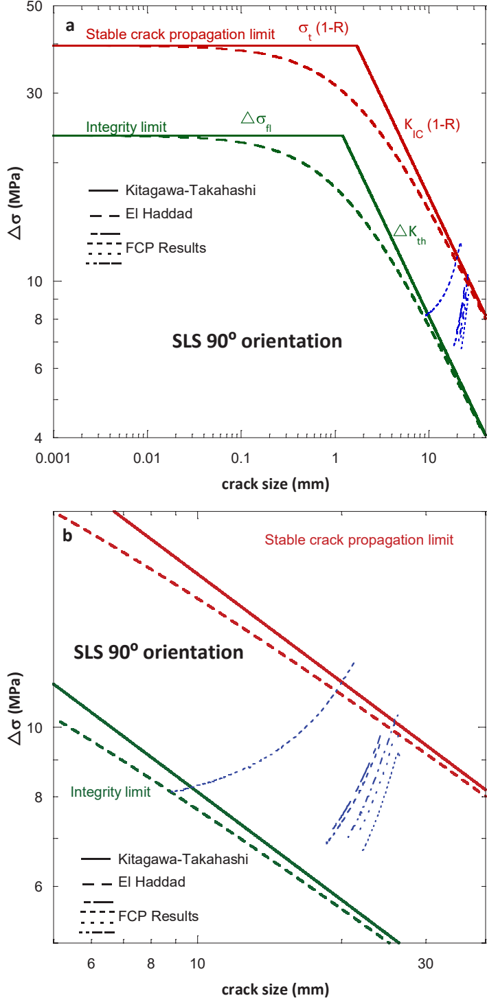
Figure 6-8. Kitagawa-Takahashi diagrams (continuous lines) including El Haddad empirical models (dotted lines) for infinite fatigue lifetime in green and for fracture at one cycle in red of SLS PA12 at 90° orientation: a) full diagrams and b) detail of LC regime with Fatigue Crack Propagation Results obtained from \Delta\sqrt{G} -increasing tests.
