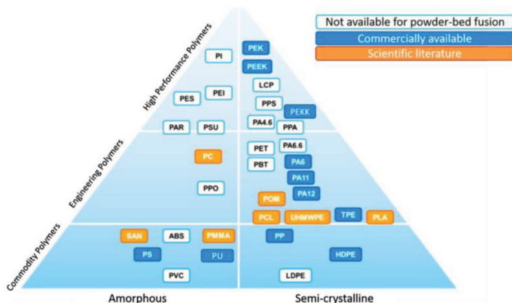
Figure 2-7. Characteristic thermoplastic polymers available for SLS process [18].
