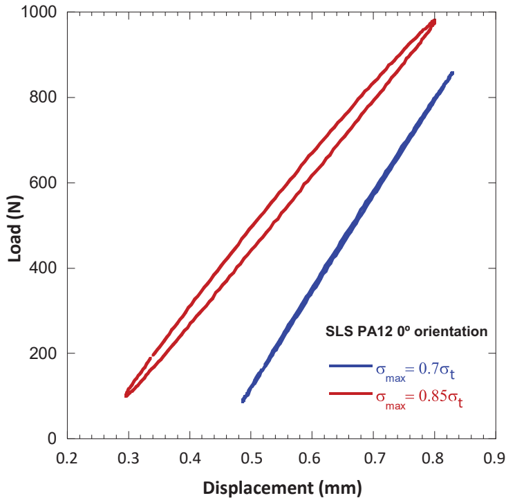
Figure 5-46. Hysteresis loops obtained from the cyclic load-displacement records of the last cycle before rupture of the tests at stress ratios of 0.7 and 0.85 performed in PA-12 at 0^\circ orientation.
